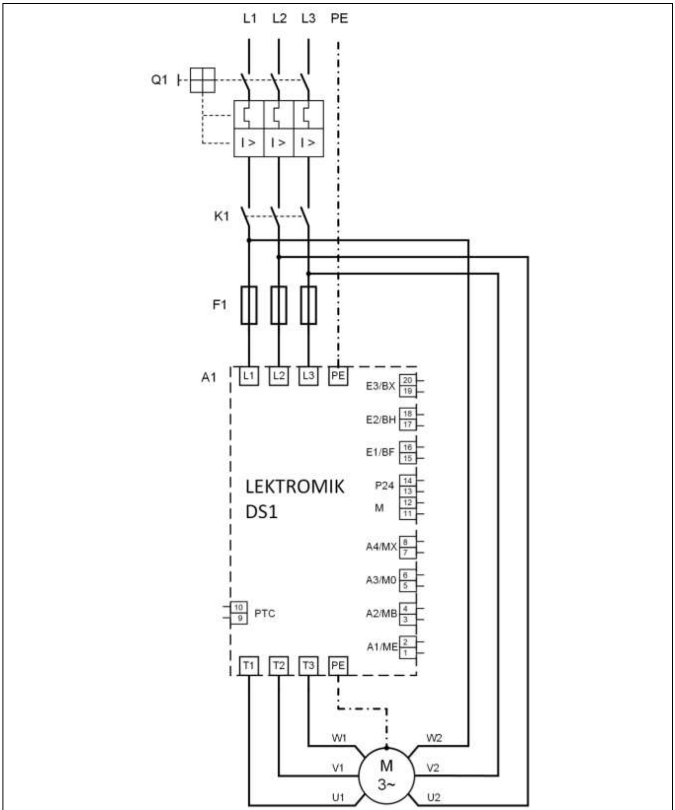
Figure 10: Connection recommendation – power circuit in delta connection
