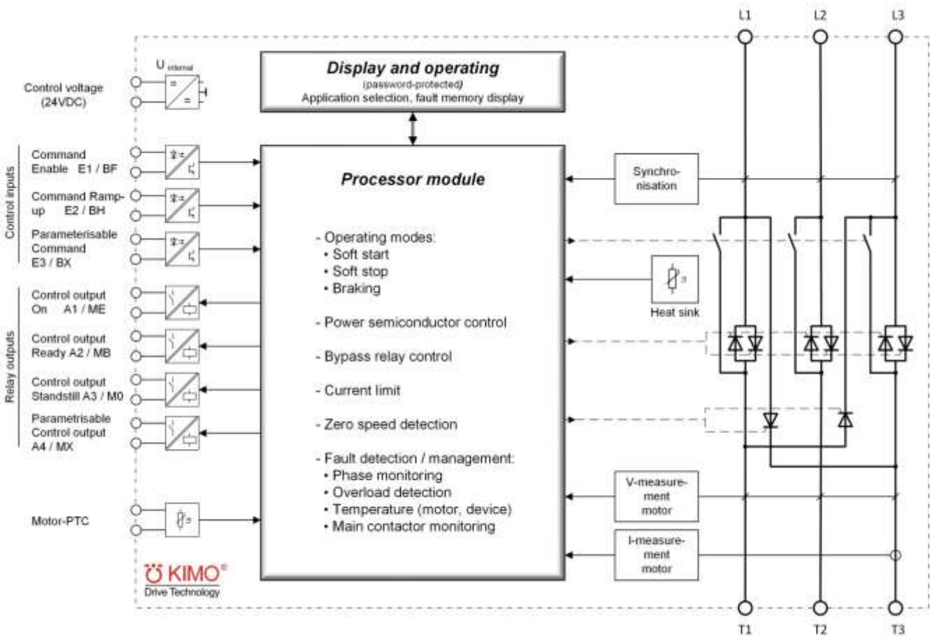
Figure 2: Block diagram
