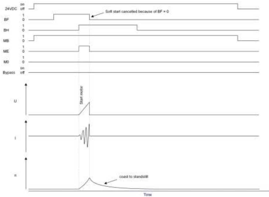
Figure 16: Condition diagram – Soft start cancelled through BF=0
