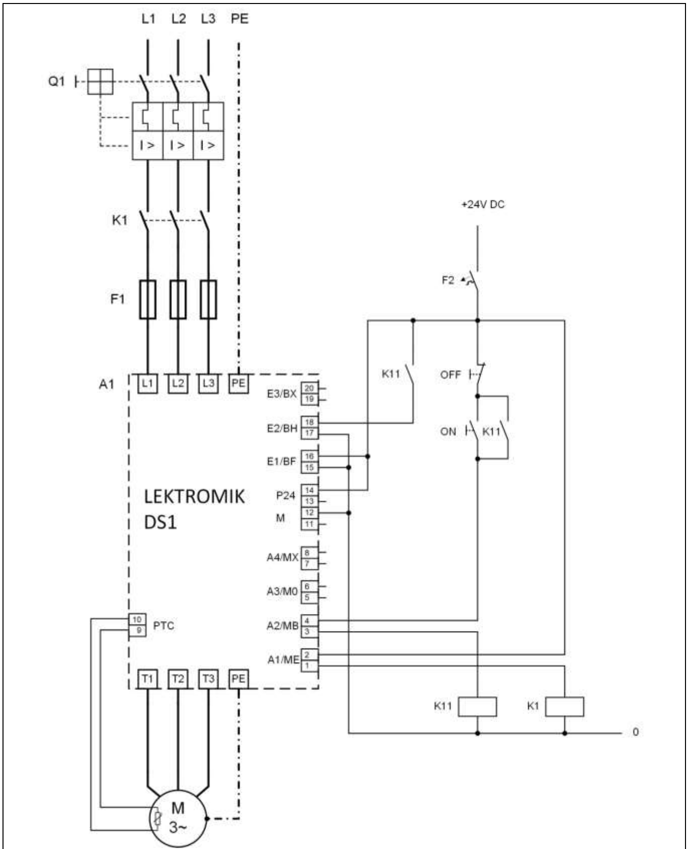
Figure 8: Connection recommendation – manual control
